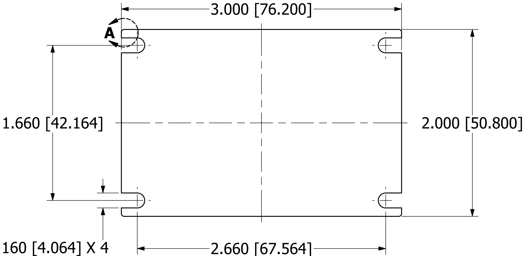
BOTTOM VIEW
